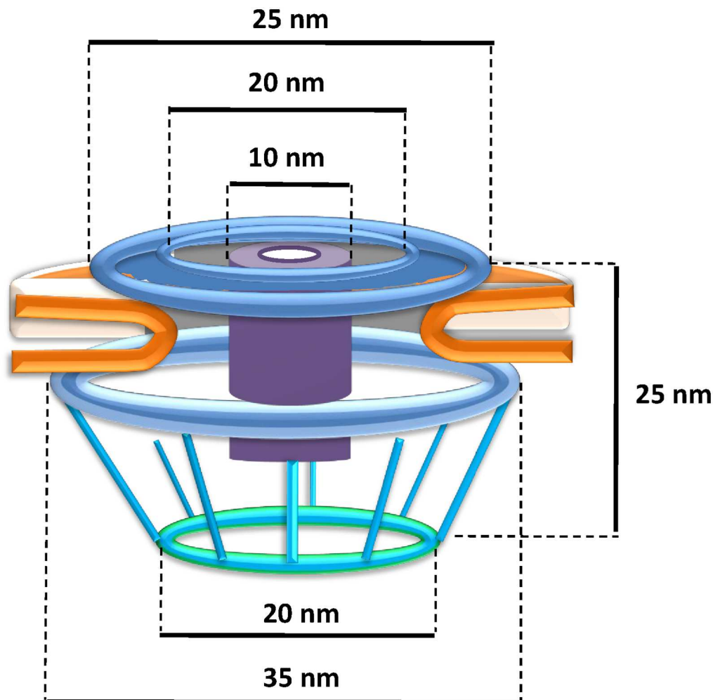
Fig 6. Model of the pore complex of Gemmata obscuriglobus . The pore complex is composed of at least two concentric upper rings (blue), and a lower ring (light blue) connected by struts to a distal ring (green) to form a basket structure. The central plug (purple) rests within the inner ring and spans the length of the pore. The whole pore complex rests within membrane (orange). The structure and dimensions are based on available data from all EM methods applied, from both whole cells and fraction 3 isolated membranes, and with minimal extrapolation, so that although the pore is probably not a hollow structure the space within the pore has not been filled in.
