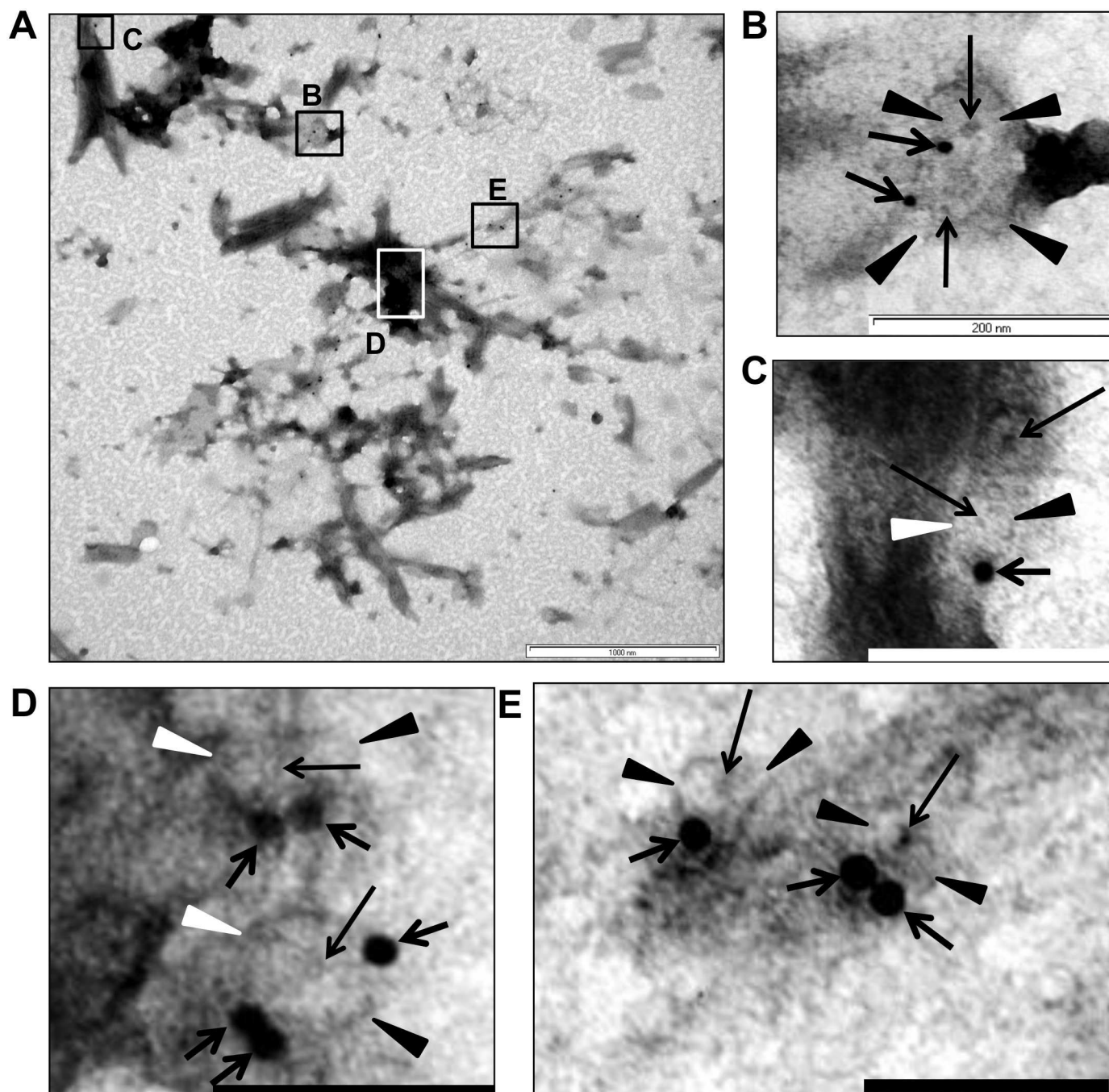
Fig 9. The antibody 6670 recognises pores in the isolated membranes. (A) Immunogold labelling of membrane sheets from membrane fraction 3 with the antibody 6670. Pellets of such fractionated membrane sheets were cryosubstituted using a protocol suitable for antigen preparation and sectioned before immunolabelling (note that the preservation of structure is not optimal in such sections due to the need for less harsh cryosubstitution conditions to allow preservation of antigenic epitopes for antibody recognition). In the majority of cases the gold particles indicating antibody can be seen as associated with the outer ring of the pores, which can be recognized in each case by a characteristic circular ring structure surrounding an electron-dense plug at their centre. Panels (B, C, D, and E) show enlarged areas of (A), which are marked as boxes in (A). In all the cases the gold particles can be seen at the edge of the pores. In some cases more than one gold particle is associated with the pores (for example see box (D), the bottom pore which is surrounded by three particles). For statistical analyses approximately the same areas were used for counting the particles: 397 particles were observed as associated with pores (distance from a pore does not exceed 20nm) and 45 particles were considered as not associated. Short thick black arrows indicate gold particles, black or white arrowheads (depending on background)—pores, and thin longer black arrows indicate the electron-dense core defining the centre of each labelled pore. Bars, A—1 \mu m, B—200nm, C, D, and E—100nm.
