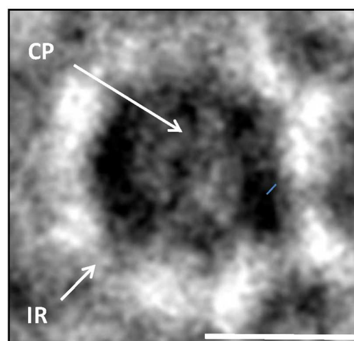
Fig 3. Pores in the membranes of Gemmata obscuriglobus released via sonication. (A) Transmission electron micrograph of a membrane fragment released from a lysed cell via sonication and negatively stained with ammonium molybdate. Large pores (arrows) with relatively electron-dense pore centers surrounded by a thin lighter inner ring and a thicker outer ring are seen. Smaller pore structures (arrowheads) are also visible and may represent either another class of pores or a result of a reverse view of the same large pores resulting from overlapping folds in the membrane (evidence for such structures
