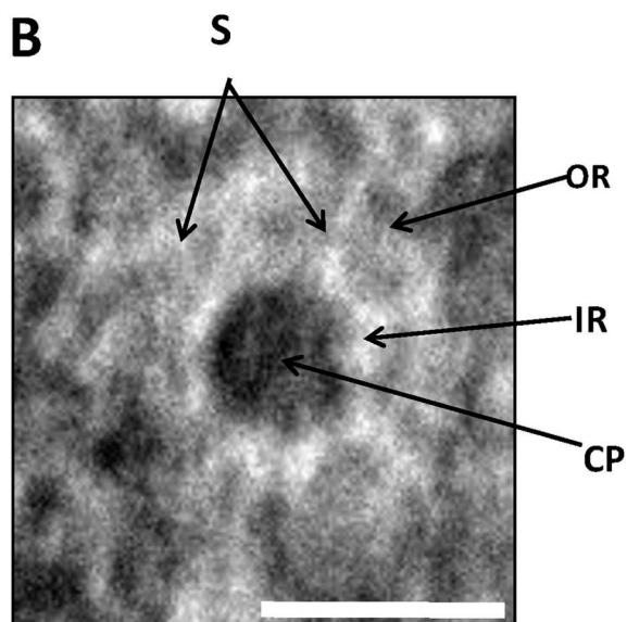
Fig 3. Pores in the membranes of Gemmata obscuriglobus released via sonication. (A) Transmission electron micrograph of a membrane fragment released from a lysed cell via sonication and negatively stained with ammonium molybdate. Large pores (arrows) with relatively electron-dense pore centers surrounded by a thin lighter inner ring and a thicker outer ring are seen. Smaller pore structures (arrowheads) are also visible and may represent either another class of pores or a result of a reverse view of the same large pores resulting from overlapping folds in the membrane (evidence for such structures
