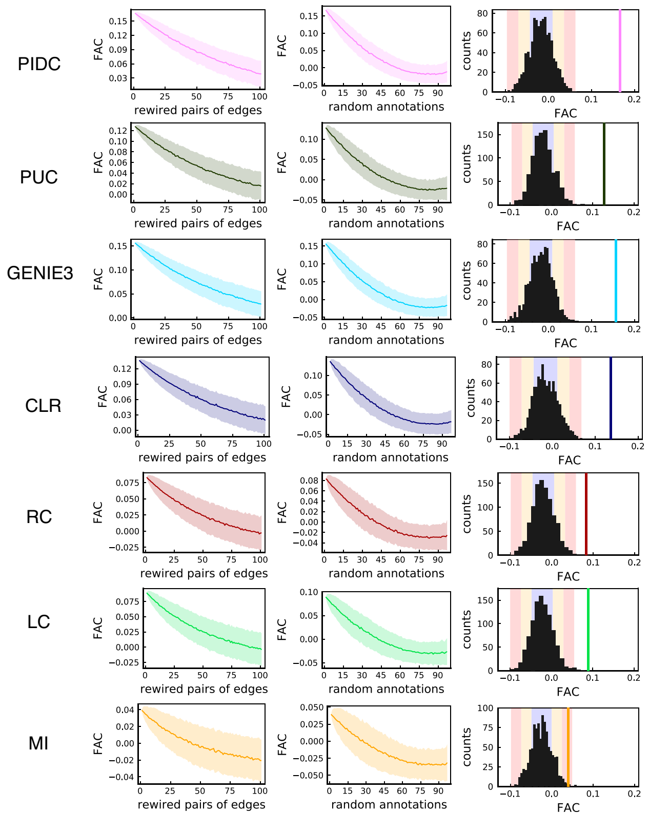
Figure 3. Illustrating the behaviour of the FAC under noisy conditions. Mean (solid line) and standard deviation from the mean (shaded area) of the FAC as pairs of edges are rewired at random (left column), and as nodes are randomly attributed a different annotation (central column)—each plot shows 1000 repeats. Right column: comparison of the observed FAC for networks with 200 edges (vertical line) against distributions of the FAC in 1000 random networks with 200 nodes; blue, orange, and red coloured bands respectively indicate one, two and three standard deviations from the mean.
