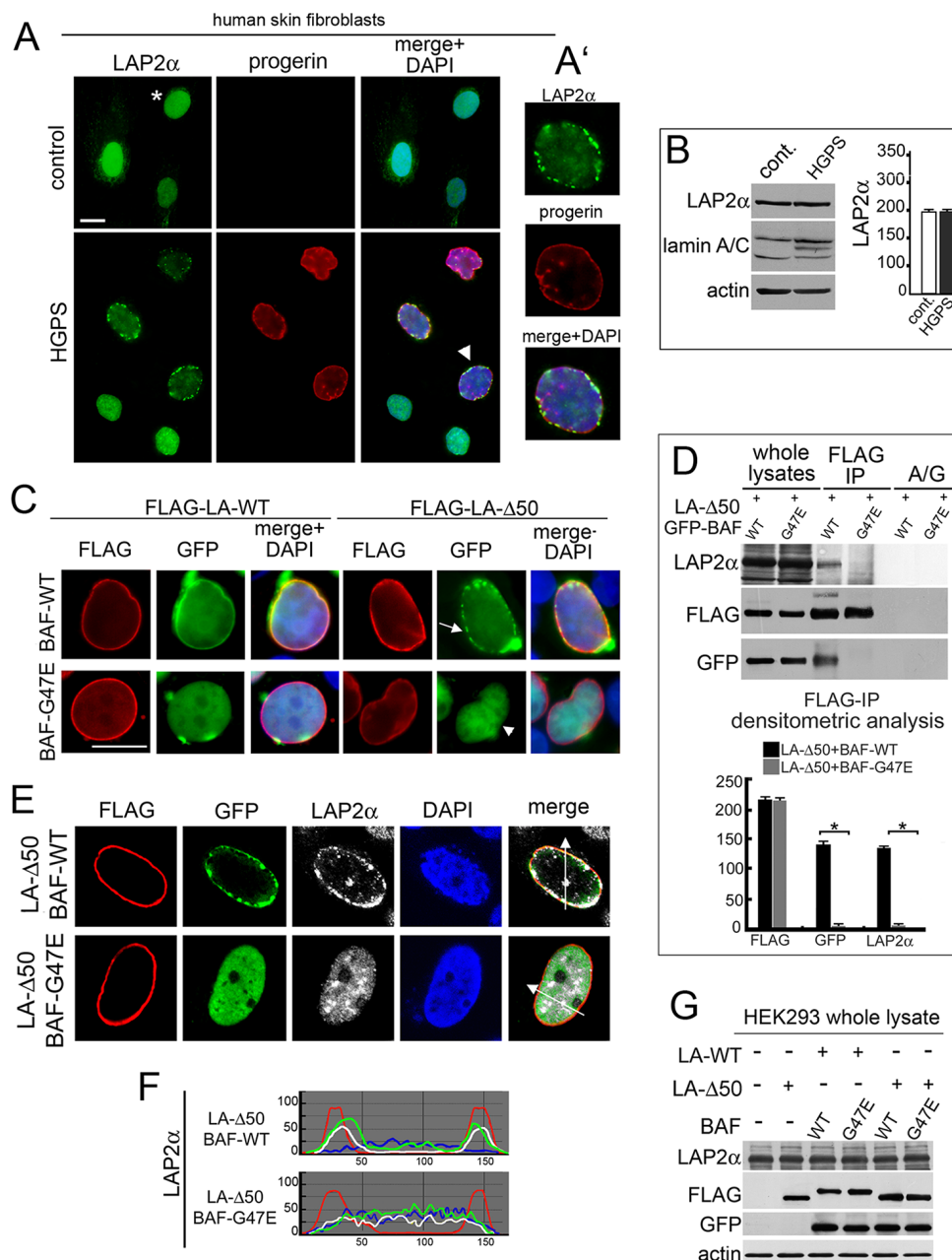
Figure 7: BAF is involved in the LAP2-alpha nuclear distribution observed in progerin expressing cells. (A) Localization of LAP2 \alpha and progerin in control and HGPS cells. LAP2 \alpha (green), progerin (red). DNA staining with DAPI is shown in merge. Bar 10 \mu m. Asterisk: LAP2 \alpha nucleoplasmic distribution. Arrowhead: HGPS nucleus shown at higher magnification in A'. (B) Western blotting evaluation of LAP2 \alpha and lamin A/C in control and HGPS cells. Actin: protein loading control. Densitometric analysis of LAP2 \alpha immunoblotted bands was performed in triplicate experiments. (C) BAF-WT and BAF-G47E localization in cells expressing LA-WT or progerin construct (FLAG-LA- \Delta 50). FLAG (red), GFP (green). DNA staining with DAPI is shown in merge. Bar 10 \mu m. Arrow: BAF-WT nuclear periphery aggregates. Arrowhead: BAF-G47E nucleoplasmic localization. Images are representative of 80% of transfected cells. (D) Western blotting evaluation of coimmunoprecipitation performed in cotransfected cells. FLAG, GFP and LAP2 \alpha immunoblotted bands obtained from whole lysates and anti-FLAG immunoprecipitation (FLAG-IP) samples are shown. No protein bands were detected in protein A/G (A/G) negative control. Densitometric analysis of FLAG, GFP and LAP2 \alpha immunoblotted bands is shown. Values are means of three independent experiments \pm S.D. (* P < 0.001). (E) LAP2 \alpha nuclear distribution in cells coexpressing LA- \Delta 50 and BAF-WT or progerin unbinding mutants BAF-G47E. FLAG (red), GFP (green), LAP2 \alpha (grey). DNA staining performed with DAPI is excluded in merge. Images shown are representative of 75% of cotransfected cells. (F) Fluorescence intensity profile along arrows drawn in (E). The top graph indicates intensity profile of BAF-WT (green), LA- \Delta 50 (red), LAP2 \alpha (white) and DAPI (blue). The bottom graph indicates intensity profile of BAF-G47E (green), LA- \Delta 50 (red), LAP2 \alpha (white) and DAPI (blue). (G) Western Blotting evaluation of LAP2 \alpha in HEK293 cells untransfected or transfected with LA-WT or LA- \Delta 50 in combination with wild type BAF (WT) or (G47E). Immunoblotted bands obtained from detection of whole lysates are shown. LAP2 \alpha , FLAG, GFP. Actin: protein loading control.
