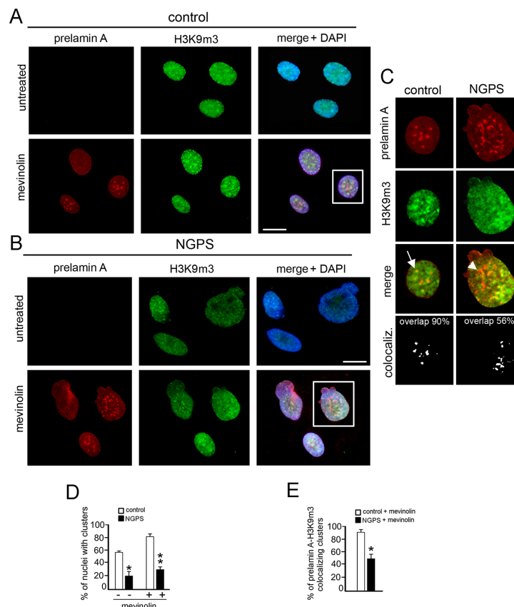
Figure 2: NGPS BAF mutation impairs prelamin A-related H3K9m3 intranuclear clustering. (A) Prelamin A (red) and histone H3 trimethylated at lysine 9 (H3K9m3, green) localization in control fibroblasts untreated or treated with mevinolin. DNA staining with DAPI is shown in merge (merge + DAPI). Bar 10 \mu M. (B) Prelamin A (red) and H3K9m3 (green) localization in NGPS fibroblasts untreated or treated with mevinolin. DNA staining with DAPI is shown in merge (merge + DAPI). Bar 10 \mu M. (C) Higher magnification of nuclei showed in A and B (squares). Prelamin A (red), histone H3K9m3 (green) and merge without DAPI staining are shown. Arrow: prelamin A-H3K9m3 costained intranuclear aggregate; arrowhead: prelamin A intranuclear aggregate in which H3K9m3 staining is missing. The percentage of prelamin A-H3K9m3 colocalized spots is reported. (D) Statistical analysis. The graph shows the percentage of nuclei showing clustered H3K9m3 in control and NGPS cells. White bars: control cells untreated (-) or mevinolin treated (+); black bars: NGPS cells untreated (-) or mevinolin treated (+). Values are means of two independent experiments \pm S.D.; for each experiment a total of 100 nuclei were considered. (* P < 0.004 ), (** P < 0.001 ). (E) The percentages of prelamin A foci colocalized with H3K9m3 are indicated. Values are means of two independent experiments \pm standard deviation. At least 100 cells were analyzed for each experiment. (* P < 0.001 ).
