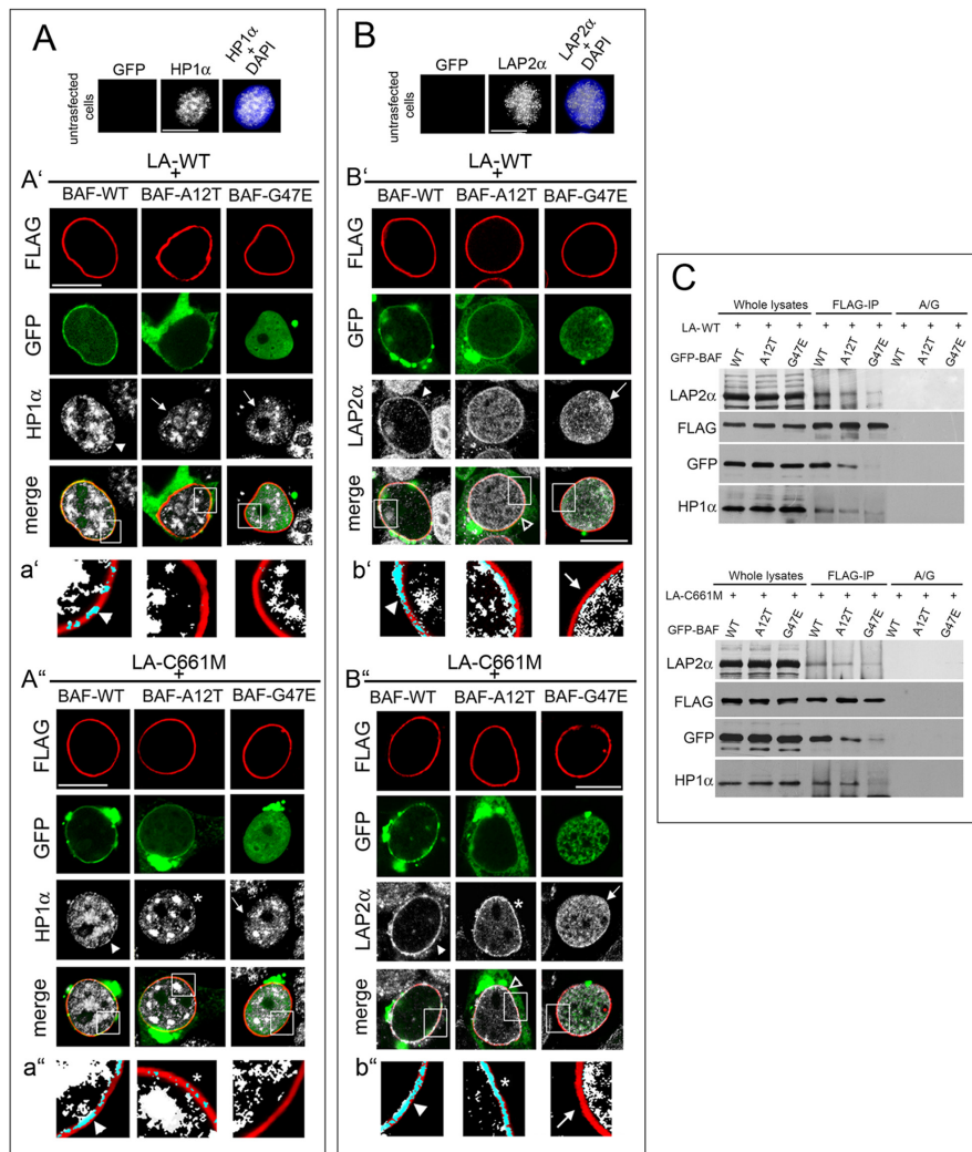
Figure 4: BAF governs HP1-alpha and LAP2-alpha nuclear relocation in prelamin A accumulating cells. (A) HP1-alpha (HP1 \alpha ) localization in HEK293 cells expressing FLAG-tagged lamin constructs in combination with GFP-BAF mutants. Top line: HP1 \alpha nuclear distribution in untransfected cells. HP1 \alpha staining (grey) is combined with DAPI (HP1 \alpha +DAPI). Bar 10 \mu M. A') HP1 \alpha localization in cells expressing wild type lamin A (LA-WT+) in combination with BAF-WT or BAF-A12T or BAF-G47E. FLAG staining (red), GFP (green), HP1 \alpha (grey). Bar 10 \mu M. a') Density dot plot of FLAG and HP1 \alpha colocalization staining showed in A'. FLAG (red), HP1 \alpha (white), merge (blue). Arrowhead: FLAG/HP1 \alpha colocalization. A'') HP1 \alpha localization in HEK293 cells expressing prelamin A (LA-C661M+) in combination with BAF-WT, BAF-A12T, BAF-G47E. FLAG staining (red), GFP (green), HP1 \alpha (grey). Bar 10 \mu M. a'') Density dot plot of FLAG and HP1 \alpha colocalization staining showed in A''. FLAG (red), HP1 \alpha (white), merge (blue). Arrowhead and asterisk indicate FLAG/HP1 \alpha colocalization. In panel (A') and (A'') arrowheads indicate HP1 \alpha nuclear periphery localization increase relative to untransfected cells (shown in top line); arrows: HP1 \alpha intranuclear localization pattern; asterisk: partial HP1 \alpha nuclear lamina localization pattern. Images shown are representative of 80% transfected cells. (B) LAP2-alpha (LAP2 \alpha ) localization in HEK293 cells expressing FLAG-tagged lamin constructs in combination with GFP-BAF mutants. In the top line LAP2 \alpha nuclear distribution in untransfected cells. LAP2 \alpha staining (grey) is combined with DAPI (LAP2 \alpha +DAPI). Bar 10 \mu M. B') LAP2 \alpha localization in cells expressing wild type lamin A (LA-WT+) in combination with BAF-WT or BAF-A12T or BAF-G47E. FLAG staining (red), GFP (green), LAP2 \alpha (grey). Bar 10 \mu M. b') Density dot plot of FLAG and LAP2 \alpha colocalization staining shown in B'. FLAG (red), LAP2 \alpha (grey), merge (blue). Arrowhead: FLAG/LAP2 \alpha colocalization. Arrow: absence of LAP2 \alpha staining at the nuclear periphery. (B'') LAP2 \alpha localization in HEK293 cells expressing FLAG-tagged wild type prelamin A (LA-C661M+) BAF-WT or BAF-A12T or BAF-G47E. FLAG staining (red), GFP (green), LAP2 \alpha (grey). Bar 10 \mu M. b'') Density dot plot of FLAG and LAP2 \alpha colocalization shown in B''. FLAG (red), LAP2 \alpha (white), merge (blue). Arrowhead; FLAG/LAP2 \alpha colocalization. Asterisk: partial FLAG/LAP2 \alpha colocalization. Arrow: absence of LAP2 \alpha staining at the nuclear periphery. In (B') and (B'') arrowheads indicate LAP2 \alpha nuclear periphery localization, arrows indicate LAP2 \alpha nucleoplasmic distribution, empty arrowheads indicate a partial LAP2 \alpha nuclear lamina recruitment, asterisk indicate a more detectable LAP2 \alpha nuclear lamina staining observed in LA-C661M+BAF-A12T expressing cells. Images are representative of 80% transfected cells. (C) LA-WT and LA-C661M coimmunoprecipitation experiment performed in cotransfected cells. Protein complexes recovered by anti-FLAG antibody (FLAG-IP) as well as whole lysates were subjected to FLAG, GFP, HP1 \alpha and LAP2 \alpha Western blotting detection. No protein bands were observed in protein A/G negative control (A/G).
