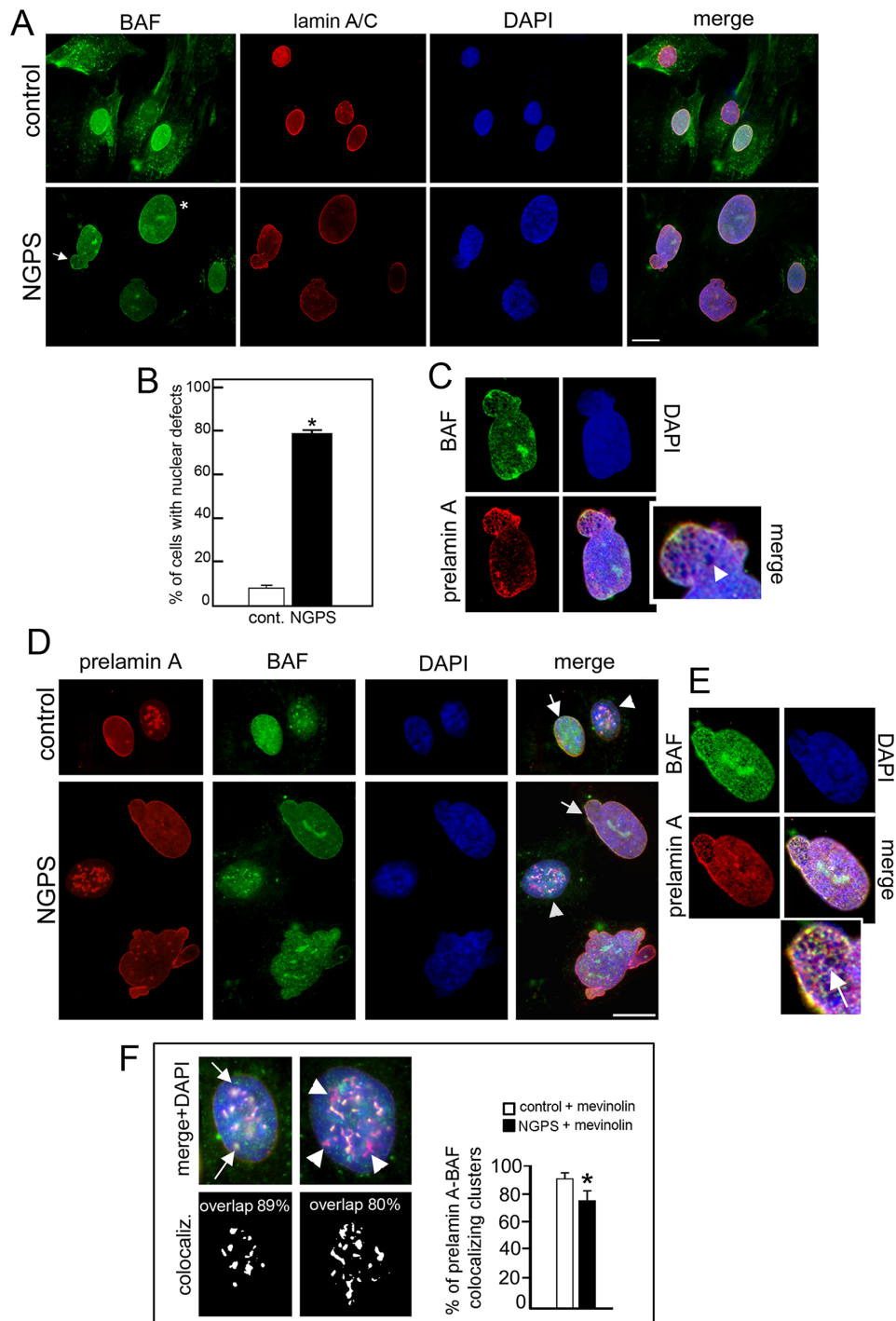
Figure 1: NGPS BAF mutation affects nuclear morphology, induces lamin A/C and prelamin A distribution defects.
