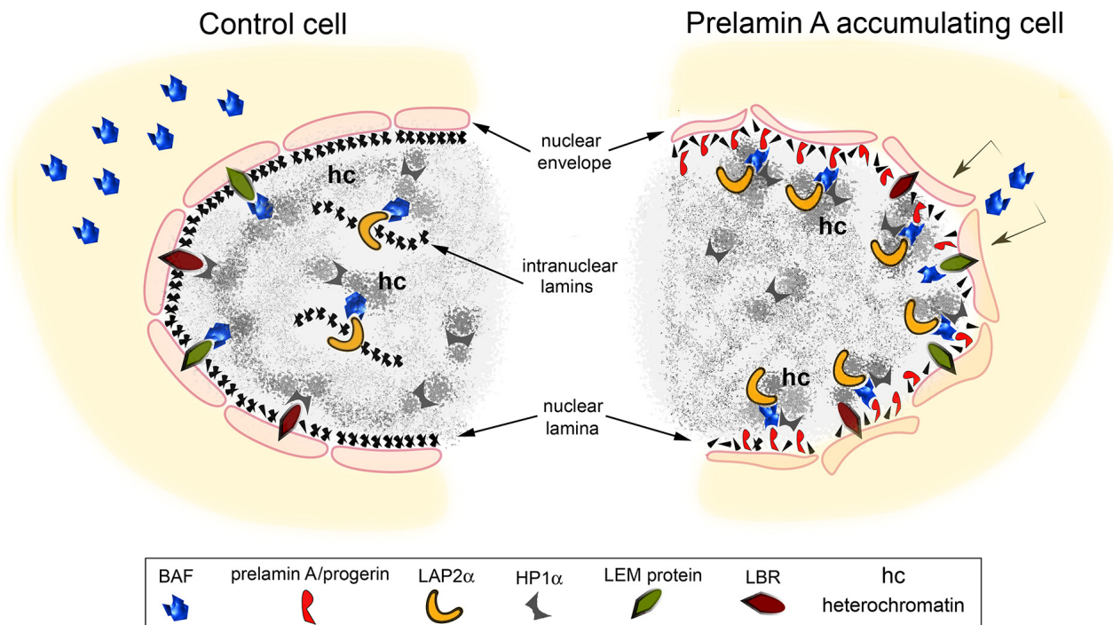
Figure 8: Speculative cartoon of the mechanism involving prelamin A-BAF interaction in chromatin organization change. In normal cells BAF localizes both at the cytoplasm and in the nucleus. At the nuclear level BAF is distributed close to the inner nuclear membrane where it interacts with LEM-proteins (LAP2, emerlin and MAN1) as well as in the nucleoplasm where it binds intranuclear form of LAP2: LAP2 \alpha . Lamin B receptor (LBR) and heterochromatin binding protein 1 alpha (HP1 \alpha ) are involved in the organization of heterochromatin. The accumulation of prelamin A/progerin affects BAF localization in the cell influencing chromatin organization. In particular, the accumulation of lamin A precursors induce BAF translocation from the cytoplasm to the nuclear lamina where prelamin A and BAF interact. BAF mediates prelamin A accumulation effects on chromatin organization. Prelamin A takes advantage of BAF interaction with DNA and DNA organizing proteins to modify chromatin organization as demonstrated by LAP2 \alpha and HP1 \alpha nuclear relocalization.
