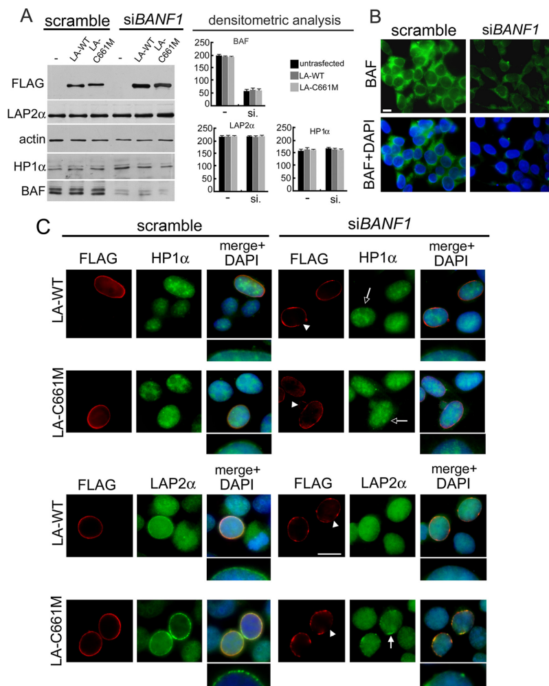
Figure 5: BAF depletion interferes with prelamin A-mediated HP1-alpha and LAP2-alpha nuclear relocation. (A) Western blotting evaluation of total lysates from HEK293 cells subjected to BAF depletion by siRNA treatment. Cells treated with scramble or BANF1 siRNA ( siBANF1 ) were untransfected (-) or transfected with LA-WT or LA-C661M constructs. FLAG, LAP2 \alpha , HP1 \alpha and BAF proteins bands are shown. Actin: protein loading control. Western blotting densitometric analysis is reported. (B) Immunofluorescence evaluation of BAF in HEK293 cells treated with scramble or BANF1 siRNA. BAF (green) and DNA staining (DAPI) are shown. Bar 10 mm. (C) Immunofluorescence detection of LA-WT, LA-C661M, HP1 \alpha and LAP2 \alpha in cells treated with scramble siRNA or siBANF1 . FLAG (red), HP1 \alpha and LAP \alpha (green). DNA was costained by DAPI and shown in merge. Arrowheads: nuclear lamina rarefaction staining of FLAG tagged proteins. Empty arrows: absence of the HP1 \alpha nuclear periphery staining increase. Arrow indicates the defective LAP2 \alpha nuclear periphery recruitment. Higher magnification of nuclear periphery distribution of HP1 \alpha and LAP2 \alpha staining, merged with DAPI, is shown. Bar 10 \mu m.
