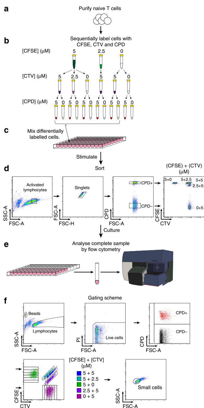
Figure 2 | A novel high-throughput clonal assay to measure T-cell division fate. (a) OT-I/ Bcl2l1 -/- CD8 + T cells were purified and (b) labelled sequentially with different combinations and concentrations of CFSE, CTV and CPD. (c) T cells from the 10 different labelling configurations indicated were mixed together and stimulated with N4 peptide ± αCD28 (2 μg ml -1 ). Between 500 and 2,000 cells from each of all 12 labelling configurations were also cultured separately to use as compensation and gating controls. (d) Just prior to first division (26 h) a single cell per labelling configuration from each stimulation condition was sorted into new wells and cultured ± hIL-2 (1 U ml -1 ). Thus there were four stimulation conditions in total: N4-only, N4 + αCD28, N4 + IL-2, N4 + αCD28 + IL-2. (e) 7,500 beads and propidium iodide (PI) were added per well before analysis to estimate sample recovery and detect dead cells. Cells were carefully transferred to tubes and the complete sample was collected by flow cytometry. Proliferation of clonal progeny cells was measured at 54, 62 and 72 h post stimulation. (f) Gates for data analysis were created using control populations at each time-point then applied to the clonal samples. FSC/SSC profile was used to gate beads and lymphocyte populations and then PI exclusion used to identify live cells. Live cells were separated out into differentially labelled populations by classifying cells as CPD + or CPD - then plotting CFSE versus CTV to distinguish the division number of cells from different labelling populations. FSC/SSC was then used to classify cells as small, thus having reached their DD (see Supplementary Fig. 2 and Methods for further details on small cell gating).
