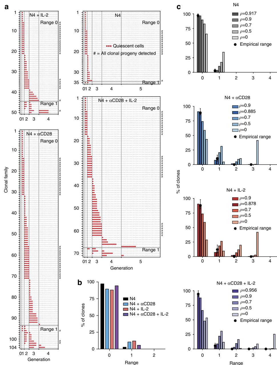
Figure 4 | Clonal family DD is highly concordant. OT-1/ Bcl2l1 -/- CD8 + T cells labelled with a division tracking dye multiplex were stimulated with N4 peptide ± \alpha CD28 (2 \mu g ml -1 ) for 26 h, sorted for one clone per labelling configuration per new well then cultured ± hIL-2 (1 U ml -1 ) as described in Fig. 2. All cultures contained S4B6 (25 \mu g ml -1 ). (a) Generation number in which progeny cells reached DD. Data pooled from 54, 62 and 72 h from families where all detected progeny were quiescent. Founder cell input after sorting was 96, 224, 96 and 224 for N4, N4 + \alpha CD28, N4 + IL-2 and N4 + \alpha CD28 + IL-2, respectively. (b) Percentage of clones with concordant (range = 0) or discordant (range > 0) DD. (c) To quantitatively question the level of familial correlation in DD required to explain the range data in b , a mathematical model was constructed and parameterized by the data and pairwise correlation, \rho , in DD fate (see Methods). The empirical range distribution for each condition (black dots within 95% confidence intervals, see Methods), in addition to model the range distribution for different values of \rho , including the per-condition best-fit. Results from a second independent experiment are shown in Supplementary Fig. 6.
