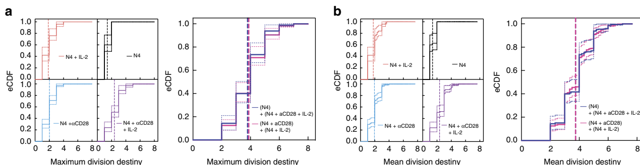
Figure 5 | Stimuli effects on DD sum independently at the level of the clonal family tree. OT-1/ Bcl2l1 -/- CD8 + T cells labelled with a division tracking dye multiplex were stimulated with N4 peptide \pm \alpha CD28 ( 2 \mu\text{g ml}^{-1} ) for 26 h, sorted for one clone per labelling configuration per new well then cultured \pm hIL-2 ( 1 \text{ U ml}^{-1} ) as described in Fig. 2. All cultures contained S4B6 ( 25 \mu\text{g ml}^{-1} ). Empirical cumulative distribution functions (eCDF) of measures of clonal expansion ( a ) maximum DD (maxDD) and ( b ) mean DD (mDD) for each individual stimulation condition (left panel). To test clonal signal addition, the convoluted distribution of the statistics from (N4) + (N4 + \alpha CD28 + IL-2) and (N4 + \alpha CD28) + (N4 + IL-2) were compared (right panel, see Methods). Vertical dashed lines represent mean of the pooled clones. Dotted lines show 95% confidence intervals. A non-standard \chi^2 -test of independence (see Methods) was not rejected for either maxDD ( P = 0.399 ) or mDD ( P = 0.237 ). Results from a second independent experiment are shown in Supplementary Fig. 7.
