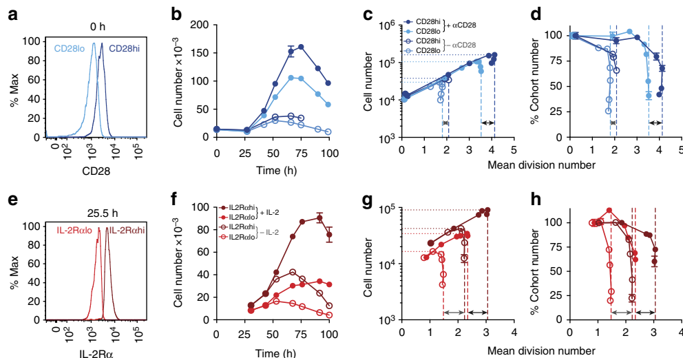
Figure 6 | Inter-clonal variation in DD is regulated by receptor sensitivity and clonal experience. (a–d) Naive CTV-labelled OT-I/ Bcl2l11 −/− CD8 + T cells were sorted into (a) CD28 high and low expressing populations and stimulated with N4 peptide ± αCD28 agonist antibody (20 μg ml −1 ). All cultures contained S4B6 (25 μg ml −1 ). Cell number versus (b) time and (c) mean division number (MDN) were measured. (d) An estimation of the percentage of the starting cells whose progeny are contributing to the response at that time point, calculated by removing the effect of cell expansion (percentage cohort number, see Methods) versus MDN. (e–h) Naive CTV-labelled OT-I/ Bcl2l11 −/− CD8 + T cells were stimulated with N4 peptide and αCD28 (2 μg ml −1 ) for 25 h then sorted for (e) IL-2Rα high or low expression. Cells were placed back into culture ± hIL-2 (3.16 U ml −1 ) and cell number versus (f) time and (g) MDN were measured and (h) percentage cohort number versus MDN calculated. Arrows indicate the difference in mDD between populations when no additional ligand (grey) or ligand at the specified concentration (black) was added to the culture. Representative of two (a–d) or three (e–h) independent experiments. Mean ± s.e.m. of triplicate culture wells.
