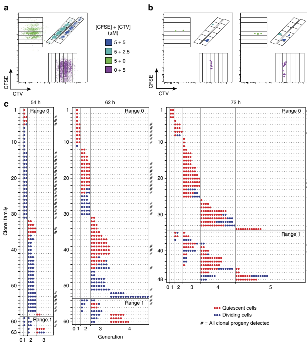
Figure 3 | Clonal T-cell family proliferation is synchronized. OT-I/ Bcl2l1 -/- CD8 + T cells were processed, stimulated and analysed as described in Fig. 2. All cultures contained S4B6 (25 \mu\text{g ml}^{-1} ). (a) N4 + \alpha\text{CD28} + IL-2 stimulated population of control cells labelled with CTV and CFSE to distinguish generation number for four distinct labelling configurations. Cells were separated into CPD + and CPD - , allowing division tracking in eight populations per well. (b) Examples of clonal progeny detected in individual wells. Example data shown for 72 h time point. (c) Generation number of progeny cells detected from individual clonal families at each time point from N4 + \alpha\text{CD28} + IL-2 stimulation condition. Progeny cells were classified as quiescent based upon small cell size (refer to Methods). Clonal range = maximum – minimum generation number. The symbol # at the end of a line denotes clones where all progeny cells were detected. Founder cell input after sorting was 80, 80 and 64 for data from 54, 62 and 72 h respectively. Results from a second independent experiment are shown in Supplementary Fig. 3.
