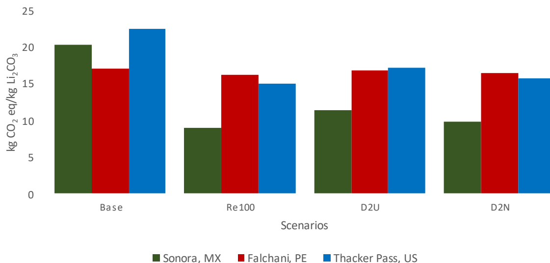
Figure 4. Sensitivity Analysis on different scenarios for Sonora, Falchani and Thacker Pass projects
