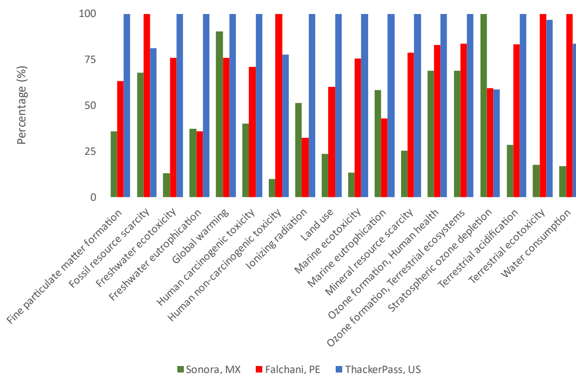
Figure 3. Comparative level of all impact categories for Sonora, Falchani and Thacker Pass
