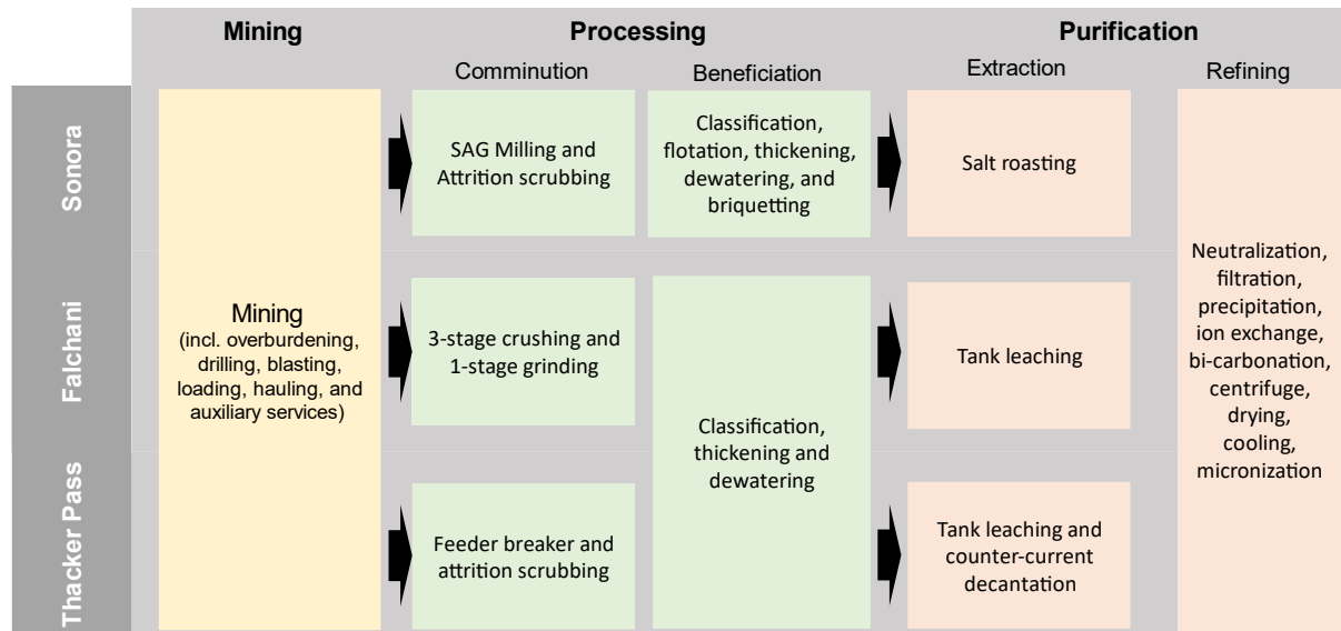
Figure 1. System flowsheet differences comparison
