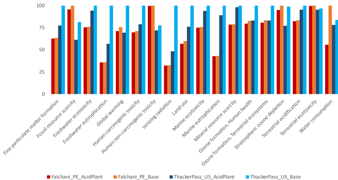
Figure 5. Sensitivity Analysis on acid plant scenarios for Falchani and Thacker Pass projects
