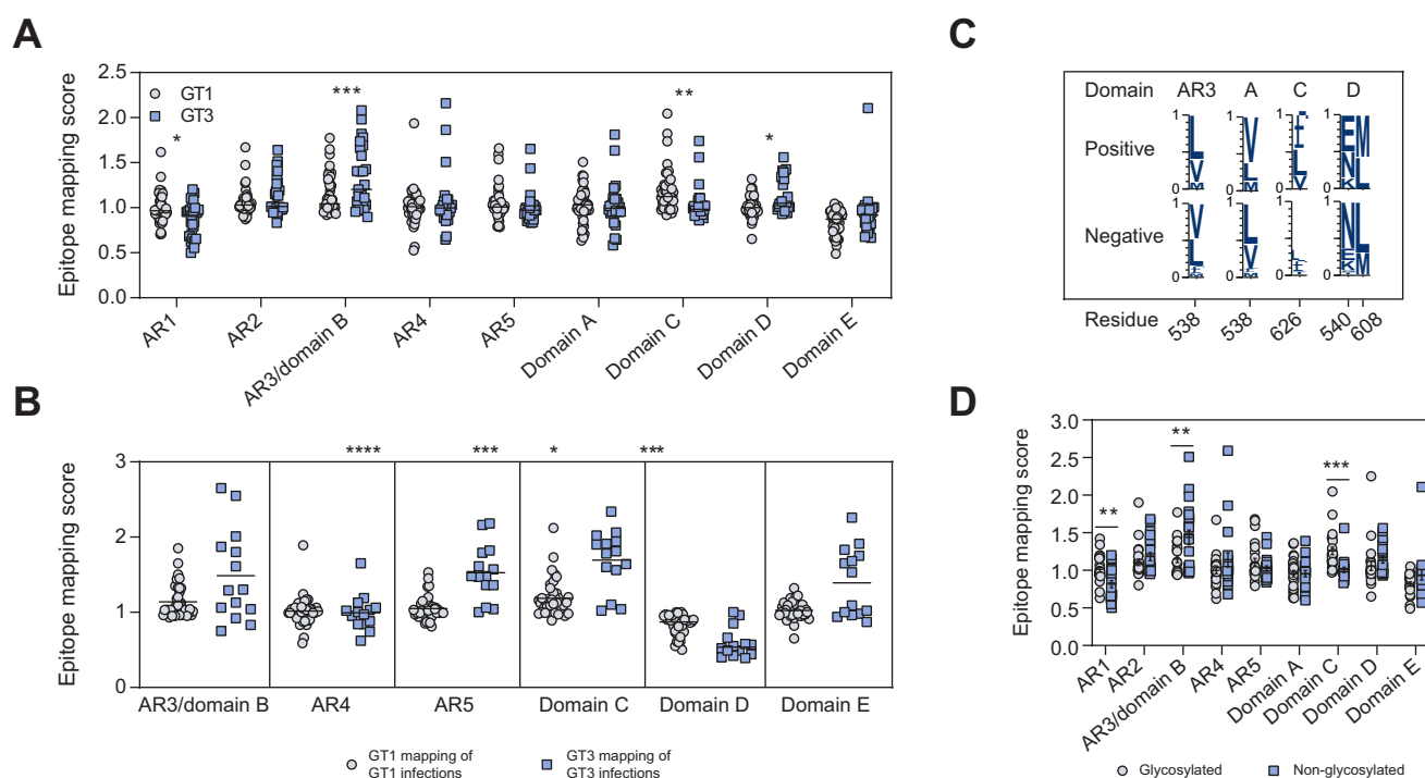
Fig. 4. Immunodominance hierarchy is associated with antigenic diversity. (A) The impact of HCV sequence on the observed GT1 epitope immunodominance was examined by comparing the specificities observed in patients infected with GT1 ( n = 43 ) to those infected with GT3 ( n = 27 ). Infection with GT3 was significantly associated with an increased response towards bNAb domains AR3 and domain D, while GT1 samples displayed a significant increase in EMS values for the narrowly neutralising domains C and AR1. (B) The EMSs of GT1-infected patients' plasma mapped to GT1 E1E2 were compared to GT3-infected patients' plasma mapped to GT3 E1E2. The results are shown for Abs against all 6 epitopes in the GT3 panel, indicating significant differences in EMS for all epitopes except those bound by AR3A and AR4A. (C) E1E2-encoding regions from 44 sequences were analysed for enrichment of amino acid residues that might be associated with epitope-specific responses. The frequency of amino acid residues that were significantly different between samples with (top) or without (bottom) epitope-specific antibodies is shown, highlighting differences in AR3 and domains A, C and D. (D) N-linked glycosylation of GT1 E2 site 540 is significantly associated with an increased dominance of domain E targeting antibodies, whereas the lack of a glycan at GT3 site 540 was associated with an increased AR3/domain B, AR5, domain C and domain D EMS (* p < 0.05 , ** p < 0.01 , *** p < 0.001 , **** p < 0.0001 , 2-tailed Mann-Whitney test). Results are shown as mean \pm SEM. AR, antigenic regions; bNAbs, broad neutralising antibodies; EMS, epitope mapping score.
