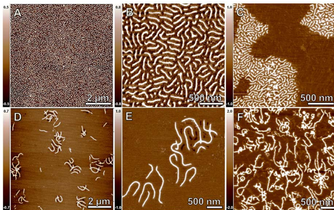
Figure 2. AFM height images of air-dried CPBs deposited from acetone on mica: (A,B) [\text{PCL}_{25}\text{-}b\text{-(PEGMA}_{98}\text{-}co\text{-GMA}_{16})]_{2700} , (C) [\text{PEGMA}_{188}\text{-}co\text{-GMA}_{32}]_{2700} , (D,E) [\text{PCL}_{14}\text{-}b\text{-(PEGMA}_{94}\text{-}co\text{-GMA}_{16})]_{7500} , and (F) [\text{PEGMA}_{170}\text{-}co\text{-GMA}_{28}]_{7500} , respectively.
