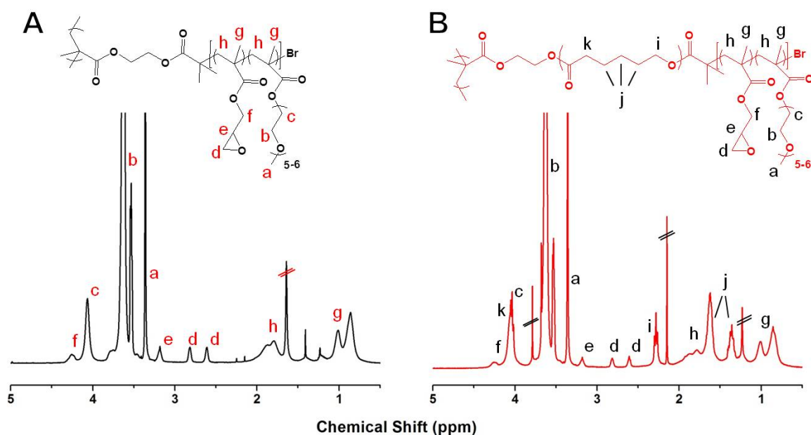
Figure 1. 1 H NMR spectra of (A) [PEGMA 140 - co -GMA 21 ] 112 and (B) [PCL 25 - b -(PEGMA 98 - co -GMA 16 )] 2700 in CDCl 3 .
