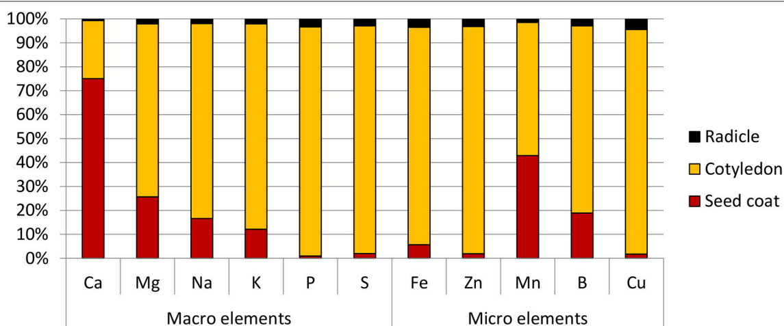
FIGURE 2 | Distribution of macro and micro elements in chickpea (cv HatTrick) seed expressed as a percentage of the total element content in the three main tissue types present in the grain. Values for the elemental profile was derived from a bulked flour sample produced from pooling tissue from 100 seeds. Three technical replicates were used. Mass distribution in the seed was calculated from 10 biological replicates.
