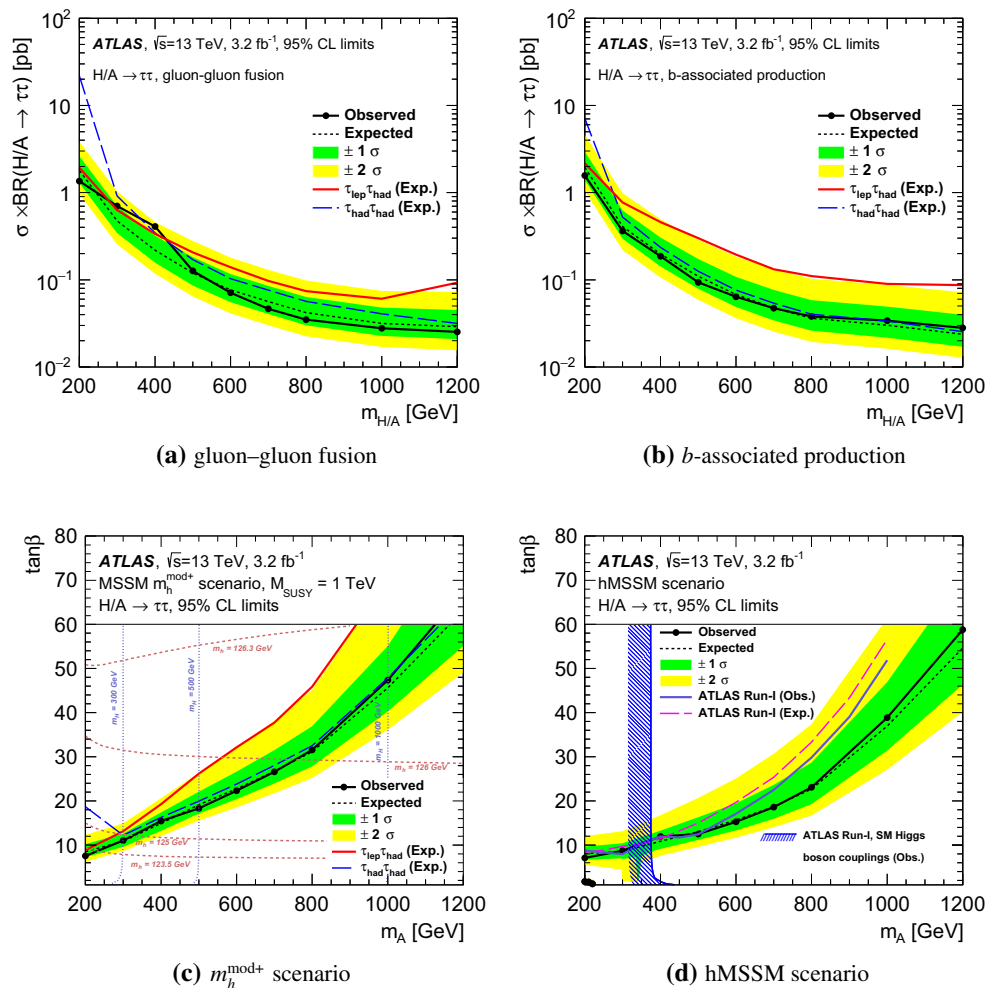
Fig. 5 The observed and expected 95 % CL upper limits on the production cross section times branching fraction of a scalar particle are shown for the combination of the \tau_{\text{lep}}\tau_{\text{had}} and the \tau_{\text{had}}\tau_{\text{had}} channels. The production mechanism of H/A \rightarrow \tau\tau is assumed to be a gluon–gluon fusion or b b -associated production. For comparison, the expected limits for the individual channels, \tau_{\text{lep}}\tau_{\text{had}} and \tau_{\text{had}}\tau_{\text{had}} , are shown as well. The observed and expected 95 % CL limits on \tan\beta as a func-
