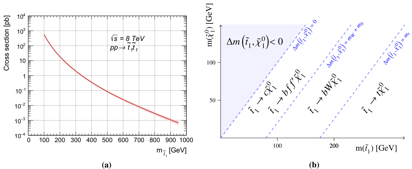
Fig. 1 a Direct stop pair production cross section at \sqrt{s} = 8 \text{ TeV} as a function of the stop mass. The band around the cross section curve illustrates the uncertainty (which is everywhere about 15–20 %) on the cross section due to scale and PDF variations. b Illustration of stop decay modes in the plane spanned by the masses of the stop ( \tilde{t}_1 ) and
