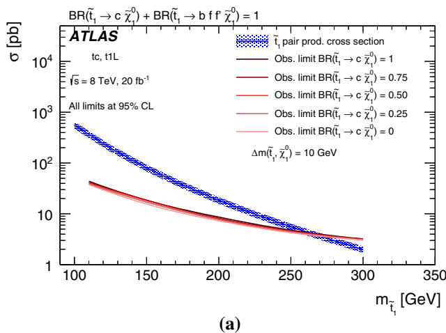
Fig. 5 Upper limits on the stop pair production cross sections for different values of the BRs for the decays \tilde{t}_1 \rightarrow c\tilde{\chi}_1^0 and \tilde{t}_1 \rightarrow f f' b\tilde{\chi}_1^0 . Signal points with \Delta m(\tilde{t}_1, \tilde{\chi}_1^0) of 10 GeV (a) and 80 GeV (b) are shown. The limits quoted are taken from the best performing, based on expected exclusion CL s , signal regions from the tc-M, tc-C, t1L-bCa_low and
