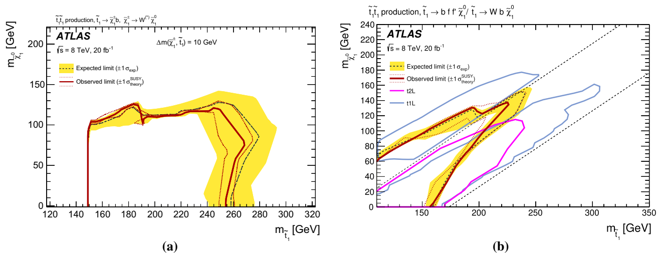
Fig. 19 Exclusion limits at 95 % CL in the scenario where both pair-produced stop decay exclusively via a \tilde{t}_1 \rightarrow b \tilde{\chi}_1^\pm followed by \tilde{\chi}_1^\pm \rightarrow W \chi_1^0 , with \Delta m(\tilde{t}_1, \tilde{\chi}_1^\pm) = 10 GeV, and b three-body or four-body decay (depending on the neutralino and stop mass). The black dashed line indicates the expected limit, and the yellow band indicates the \pm 1\sigma uncertainties, which include all uncertainties except the
